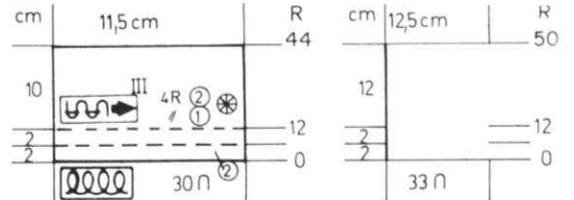
PULLOVER SLEEVES: III
