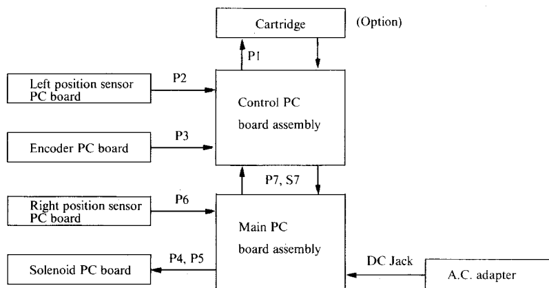
Fig. 5-1 shows the circuitry configuration of the KH-270
