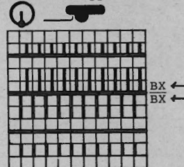
Diagram for neckband [Knit Tech 181, but with pushers on back bed all in Working Position, black strippers]
