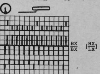
Diagram 2 for rose [Knit Tech 171, but needle, pusher and lock settings on back bed acc to this diagram. Note : orange strippers]
