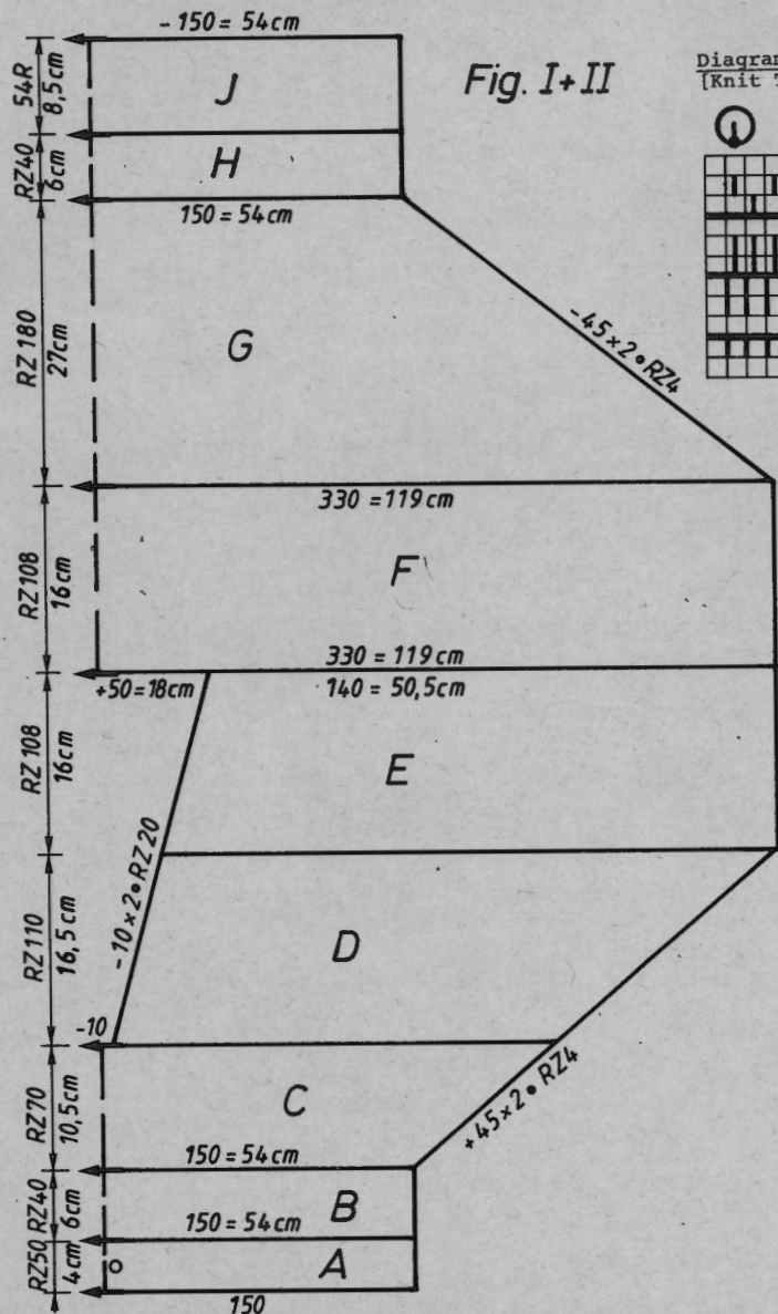
Chart for deco card
