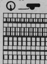
Diagram 2 for neckband [Knit Tech 181, but pushers on back bed all in WP, black strippers]
