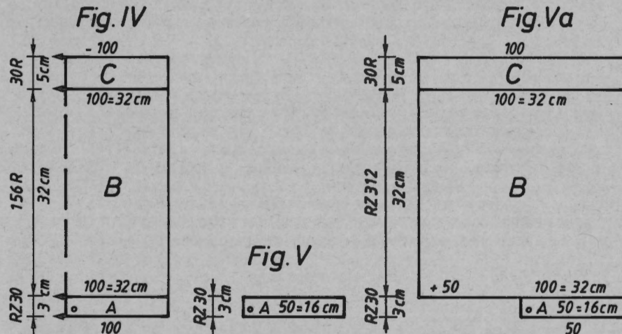
Diagram for intarsia [TECH 245]
