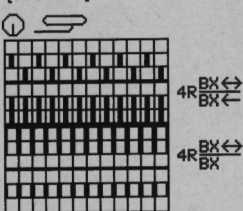
Diagram 2 for plain Fairisle [TECH 207]
