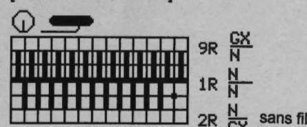
Diagram for release pattern [ELECTRONIC as well]
