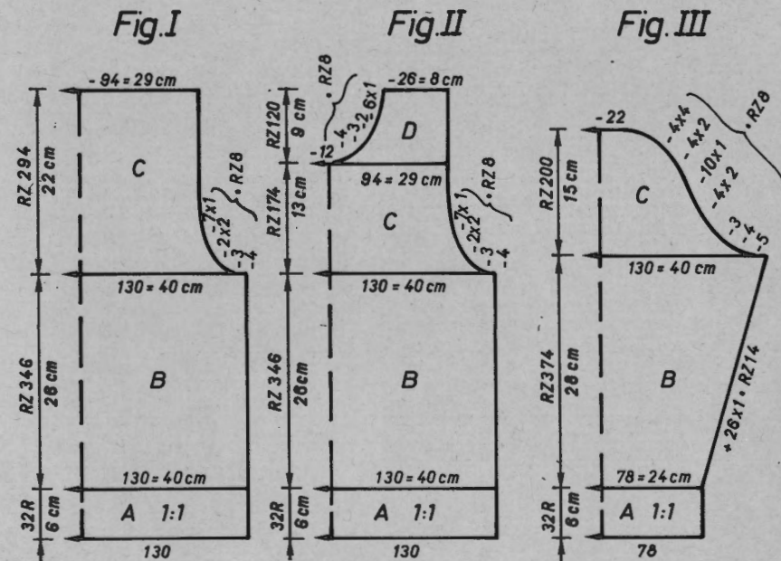
Diagram for 4 colour Fairisle [TECH 209]
