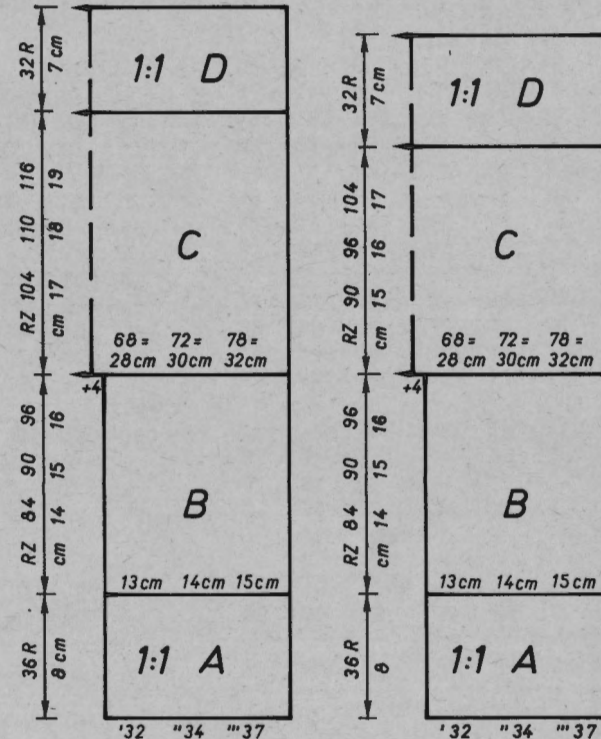
Diagram 1 for tuck stitch pattern single bed [pattern 1000, TECH 169]
