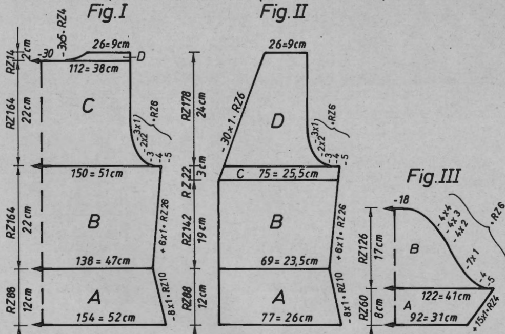
Diagram for Technique 195 (Rear pushers and lock position according to diagram and not according to indicator.)
